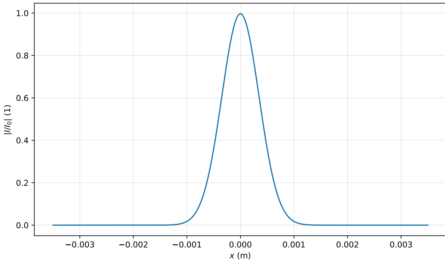
Intensity profile I(x, y = 0, z = 0.239m)/I_0 , P_{in}=0.2P_{cr} , artificial time
